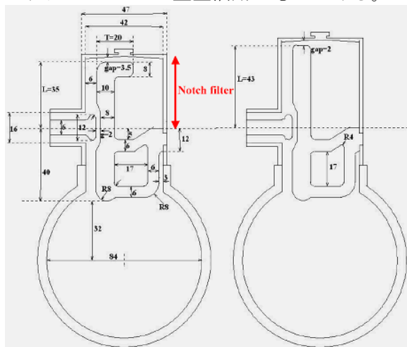
(a) KEK L-type (b) KEK I-type
