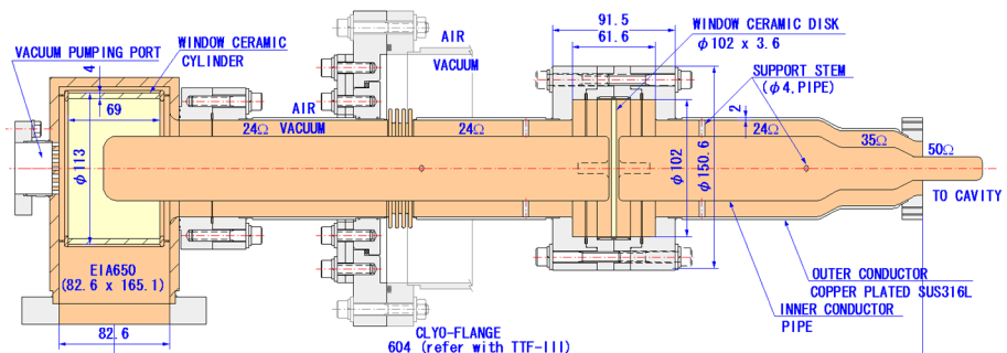
Figure1: A first prototype of input coupler for the ILC 45MV/m version cavity.
