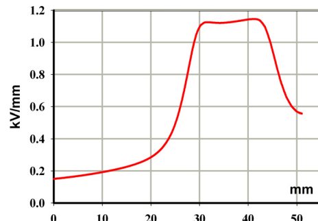
Figure 6: Electrical field distribution on the ceramic surface.
