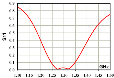
Figure 9: Frequency pass-band of cold window.
