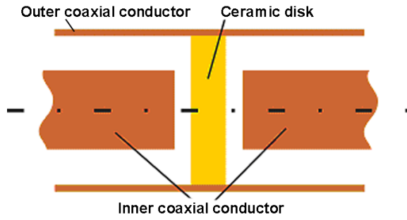
Figure 2: Conceptual sketch of the capacitive coupling for the rf window.
