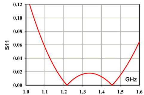
Figure 5: Frequency pass-band of the rf window.
