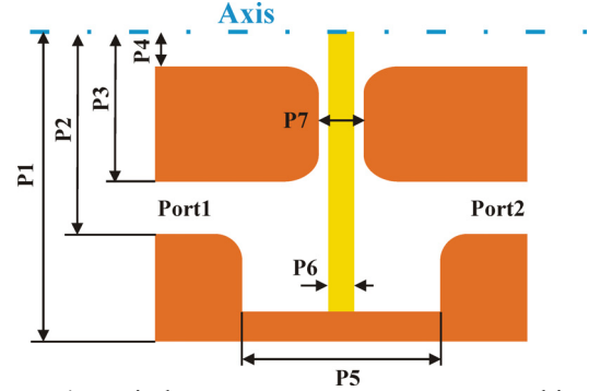
Figure 4: Window geometry parameters subject to optimisation
