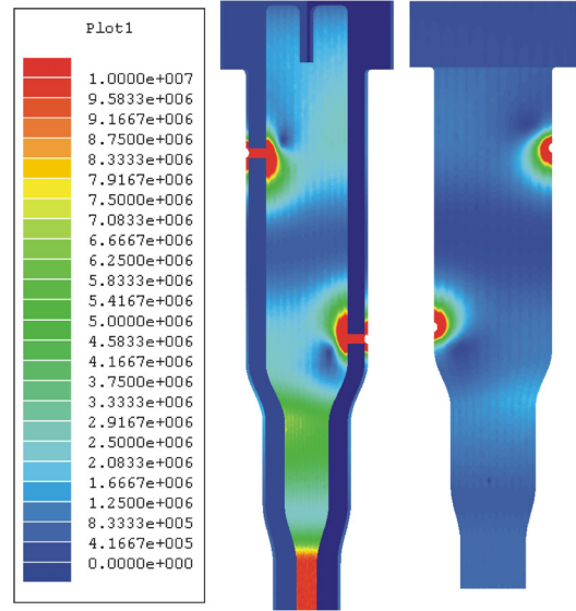
Figure 10: Distribution of magnetic field strength squared on the surface of part of the coupler.
