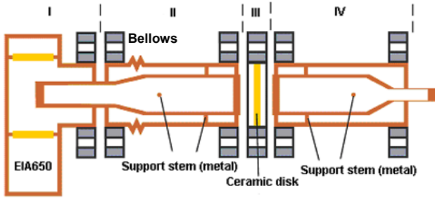
Figure 3: Over all conceptual drawing of the capacitive coupling type coupler.
