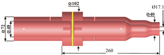
Figure 8: A cut away view of the cold window.
