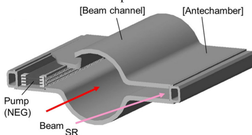
Figure 6: Sketch of the beam pipe of SuperKEKB.
