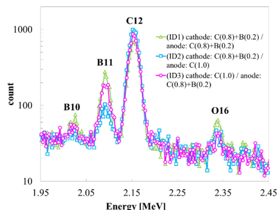
Figure 4: Comparison of RBS spectra between ID1, ID2 and ID3.
