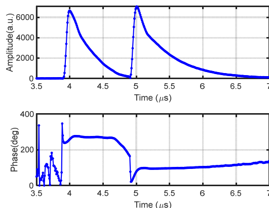
Figure 3: Reflection wave form of the RF gun.
