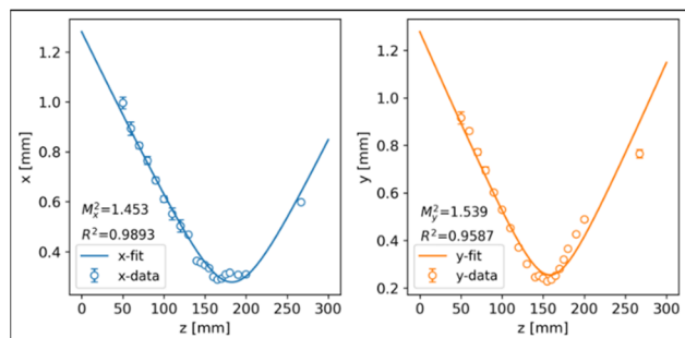
Figure 9: Result of the M^2 measurement.
