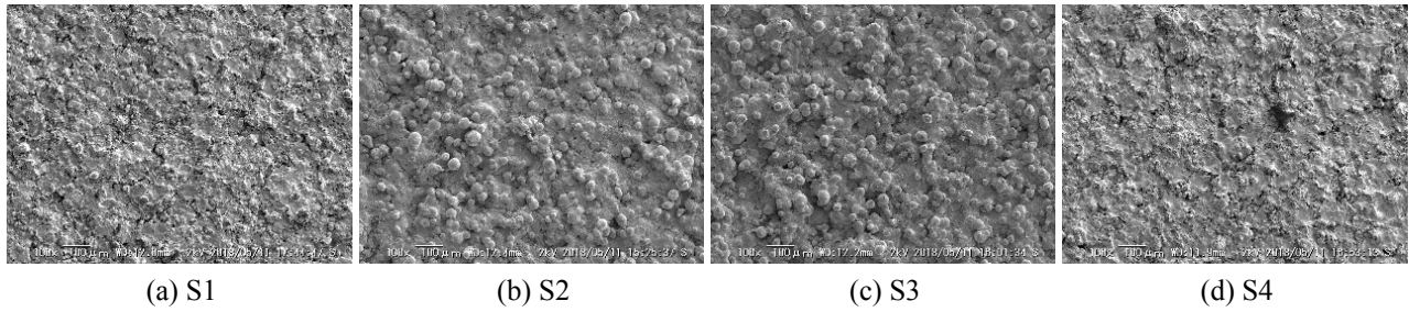
Figure 4: SEM micrographs (×100) of samples (a) S1, (b) S2, (c) S3 and (d) S4.
