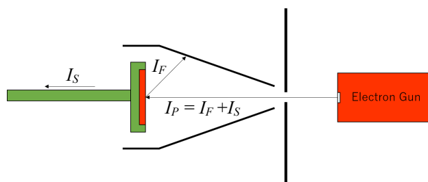
Figure 1: The schematic layout of the facility for SEY measurement.
