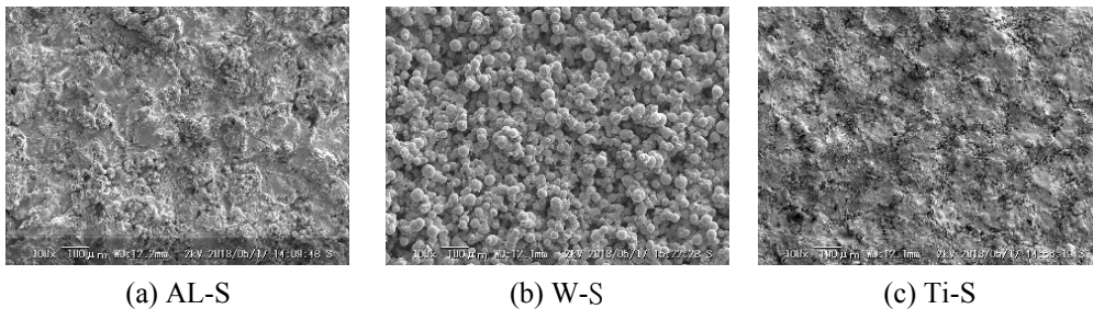
Figure 6: SEM micrographs (×100) of samples (a) AL-S, (b) W-S and (c) Ti-S.
