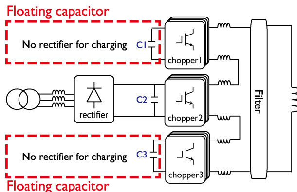
Figure 1: Schematic view of a power converter with the floating capacitor scheme.
