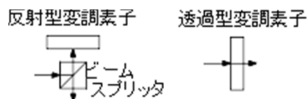
Figure 4: Generation by spatial modulator.
