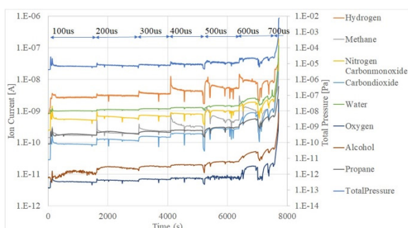
Figure 10: Trend of ion current of residual gas in the graphene irradiation test.
