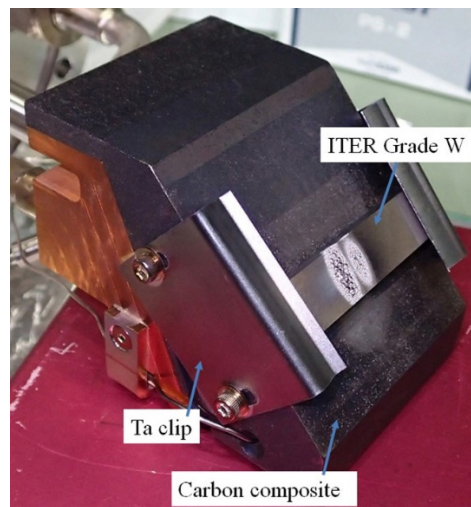
Figure 11: The photograph of the tungsten test pies on the scraper head.
