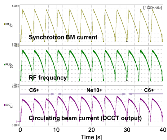
Figure 5: Operation test of multi-ion acceleration switching ion species of injection beams between ^{12}\text{C}^{6+} and ^{20}\text{Ne}^{10+} .
