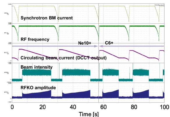
Figure 6: Operation test of multi-ion extraction for ^{12}\text{C}^{6+} and ^{20}\text{Ne}^{10+} beams.
