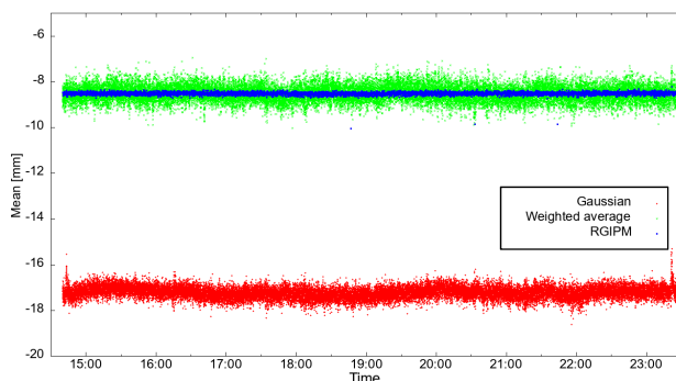
Figure 5: Trend graph of horizontal beam position at beam dump during 37-kW beam operation. Green, blue and red point illustrate the beam positions of weighted average, RGIPM and Gaussian fit respectively.
