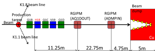
Figure 3: Schematic diagram of the primary beam line at J-PARC Hadron experimental facility. Red box and dark red boxes illustrate beam dump and RGIPMs respectively.
