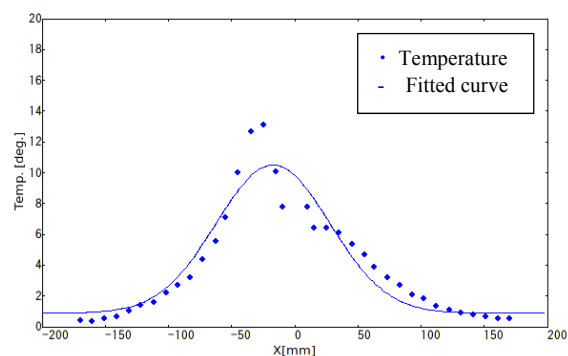
Figure 4: Typical graph of horizontal temperature distribution at beam dump during 37-kW beam operation.
