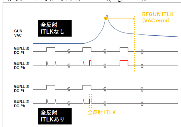
Figure 10: Consideration of total reflection.
