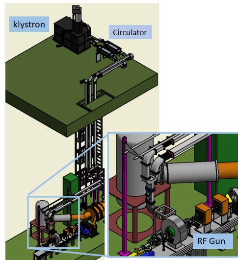
Figure 1: RF system for RF gun.
