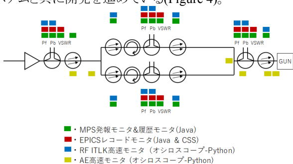
Figure 2: Monitor system for RF gun.
