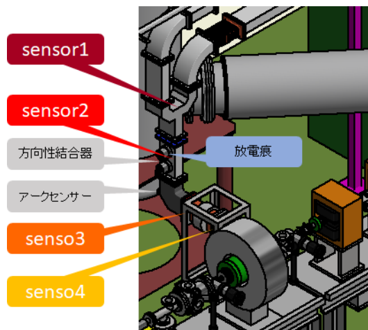
Figure 9: Position of AE sensor.
