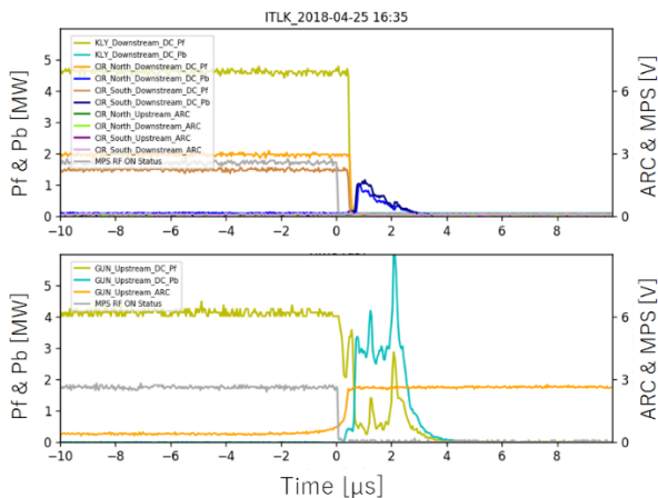
Figure 7: Waveform of RF and discharge.
