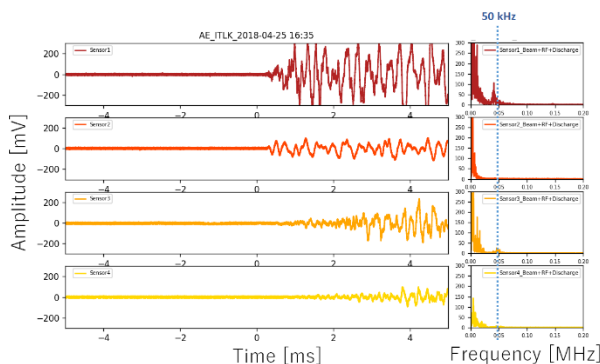
Figure 8: Waveform of AE.
