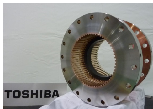
Figure 1: A completed prototype HOM absorber.
