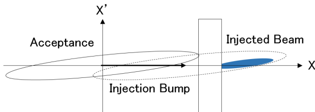
Figure 4: Horizontal phase space plots of injected beam and stored beam of Fig. 3.
