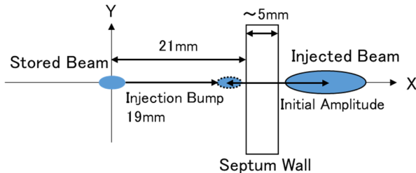
Figure 3: Injected beam and stored beam relative position at the injection point.
