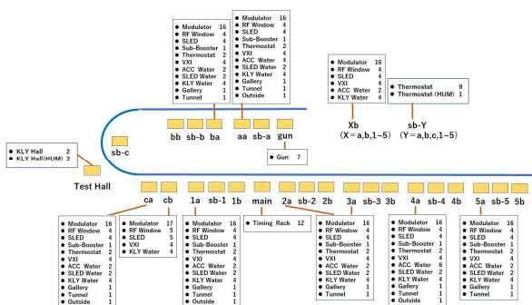
Figure 2: Schematic layout of data loggers of the temperature and humidity measurement system at the KEK injector linac.
