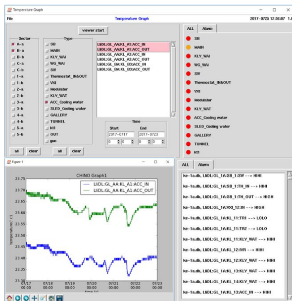
Figure 5: Image example of the new archiver data viewer and alarm display panel for managing temperature and humidity at the KEK injector linac.
