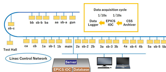
Figure 3: Schematic layout of data acquisition software for the temperature and humidity measurement system at the KEK injector linac.
