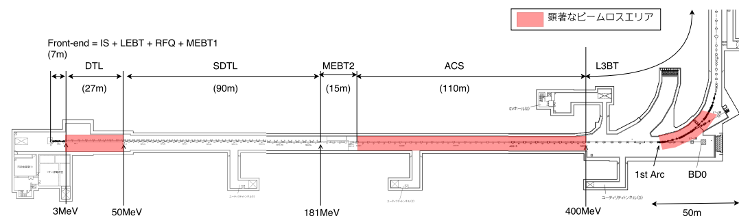
Figure 1: Severe beam loss sections between Linac and L3BT in J-PARC.
