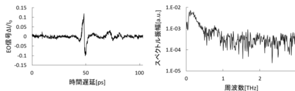
Figure 6: Results of THz pulse measurement by TDS (left: time domain, right: frequency domain).
