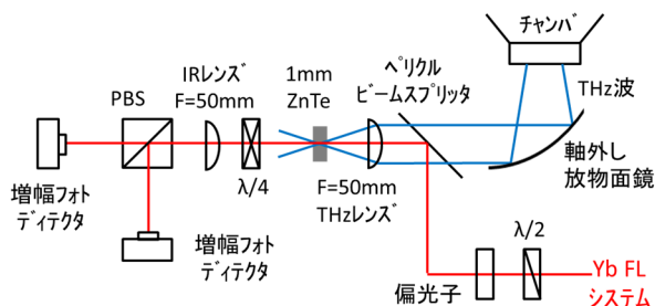
Figure 5: Setup of EO sampling measurement for THz pulses.
