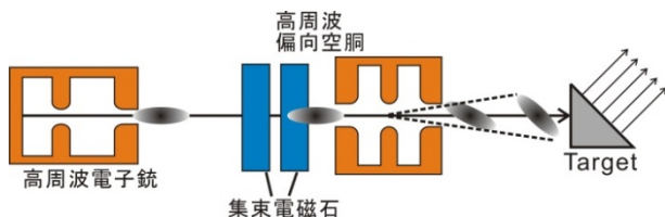
Figure 2: Beam line layout of coherent Cherenkov radiation experiment at Waseda University.
