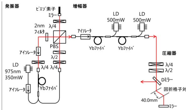
Figure 4: Setup of Yb fiber laser system for EO sampling.
