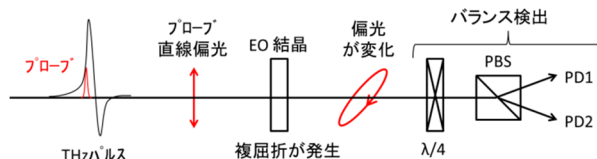
Figure 3: Schematic of EO sampling.
