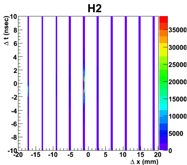
Figure 2: Residuals of x (mm) and time (ns) of fiber hits with respect to fitted tracks at Plane H2.
