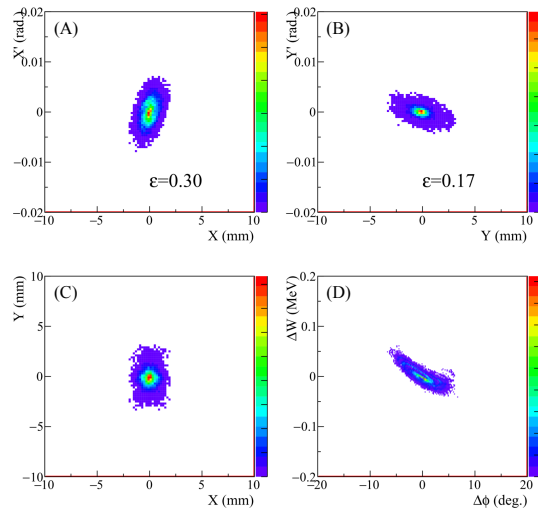
Figure 6: Simulated particle distribution at the DTL exit. (A) the horizontal divergence angle x' vs x , (B) the vertical divergence angle y' vs y , (C) y vs x , and (D) \Delta W ( W=4.2 MeV) vs \Delta\phi .
