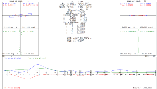
Figure 3: Matching design of the DTL using TRACE3D.
