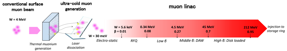
Figure 1: Configuration of low-emittance muon beam.
