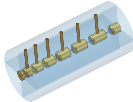
Figure 4: Three-dimensional model of DTL cavity in CST MW Studio calculation.
