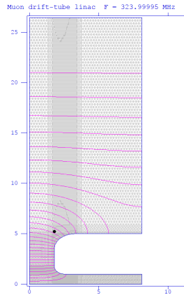
Figure 2: Electric field calculated by SUPERFISH.
