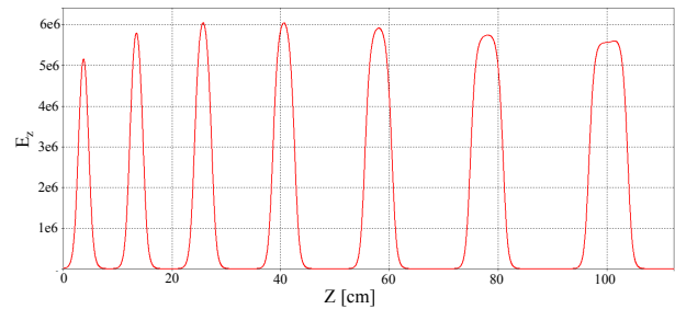
Figure 5: Longitudinal electric-field profile along the cavity.
