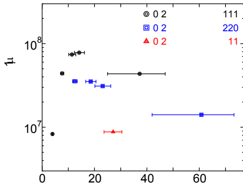
Figure 7: The PXR yield normalized by of 1- \mu\text{A} electron beam as functions of the PXR center energy.
