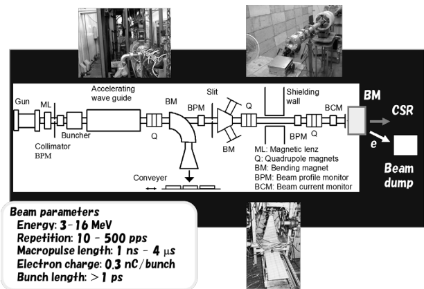
Figure 3: Schematic diagram of the OPU electron linac.
