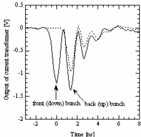
Figure 4: Outputs of the current transformer
