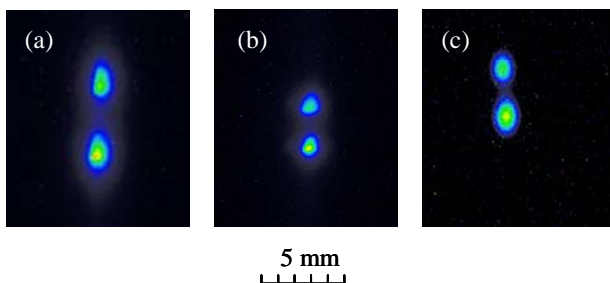
Figure 3: Double-decker electron beam profiles at exits of the rf gun (a), the linac (b) and the bunch compressor (c).
