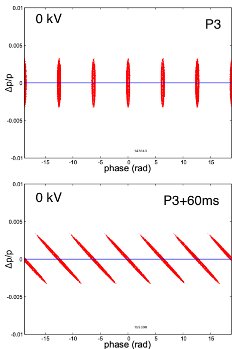
Figure 7: Beam debunched turning off the RF voltage by one step.
