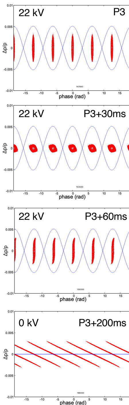
Figure 8: Beam debunched turning off the RF voltage by one step.
