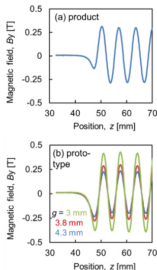
Figure 2: Magnetic fields of (a) the product and (b) prototype with three different gap lengths.
