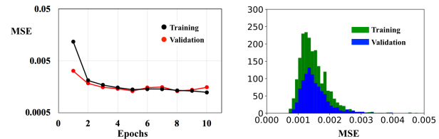
Figure 3: Learning curve and histogram of mse values.
