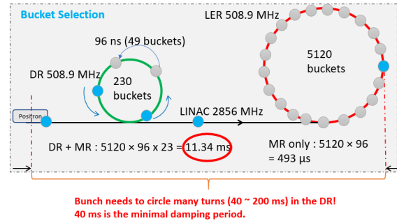
Figure 3: The synchronization between DR and LER. The positron beam is injected into the DR first and cycle for at least 40 ms. The bunch extracts from DR later and injects to the LER bucket.
