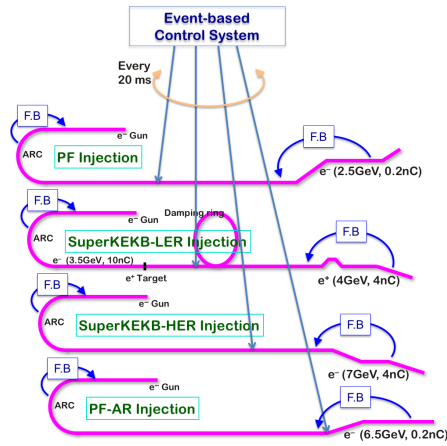
Figure 2: Pulse-to-Pulse Modulation.
