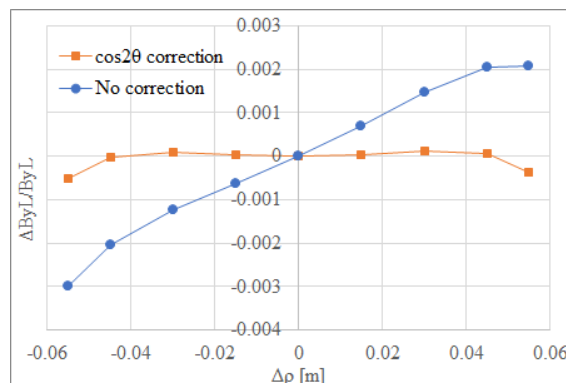
Figure 6: Uniformity of the ByL , dByL/ByL . By adding \cos 2\theta correction, quadrupole components are sufficiently corrected.
