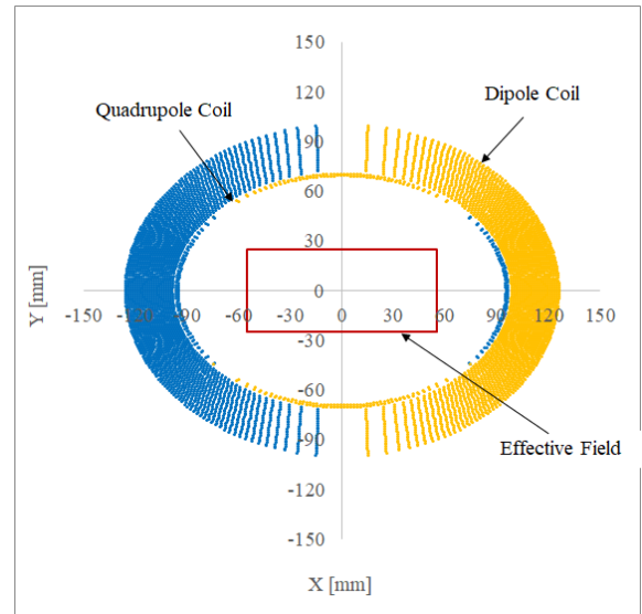
Figure 2: Cross section of the superconducting coil. A dipole and quadrupole coils are wound concentrically.
