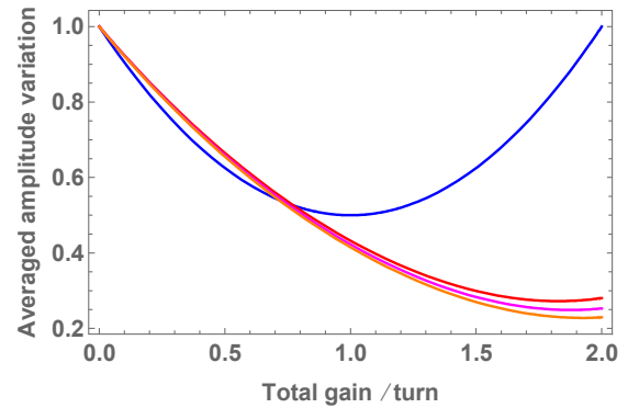
Figure 10: Averaged betatron amplitude variation with single (blue) or twin (red, magenta and orange) intra-bunch feedback systems. Curves with red, magenta and orange colors correspond to betatron tunes, 21.5, 21.25, 21.0.
