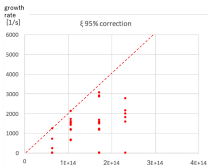
Figure 9: Growth rate measured with 95% \xi correction.
