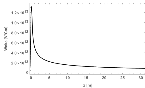
Figure 1: Resistive wall wake potential of the SUS316L vacuum duct, modeled with a cylindrical pipe of inner diameter 160 mm, thickness 2 mm, and length 1567.5 m.
