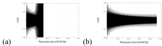
Figure 11: Stability vs processing clock frequency. Multiplication factors of 64 (a) and 128 (b) of the acceleration RF clock (simulation).
