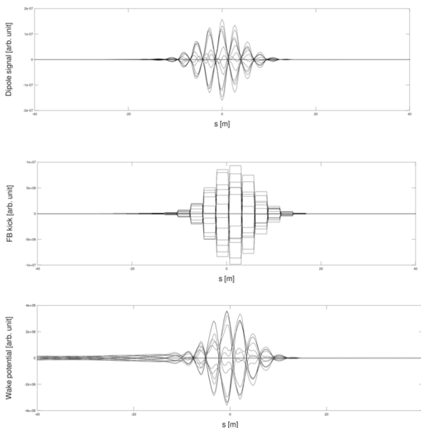
Figure 12: Dipole signals (upper), feedback kick signals (middle) and wake (lower) with the processing clock of 64 multiple of the acceleration RF clock, overlap of 13 turns (simulation).
