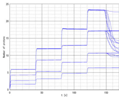
Figure 7: Beam intensity variation. Several shots are overlapped in the figure.
