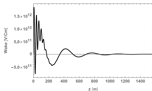
Figure 2: Wake model of the five fast-extraction kickers.
