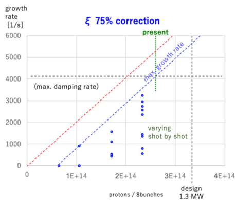
Figure 8: Growth rate measured with 75% \xi correction.
