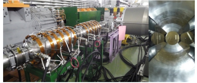
Figure 5: Stripline kickers for the intra-bunch feedback system in the J-PARC MR. The right photograph shows the vacuum side, DLC-coated electrodes and pipe wall.
