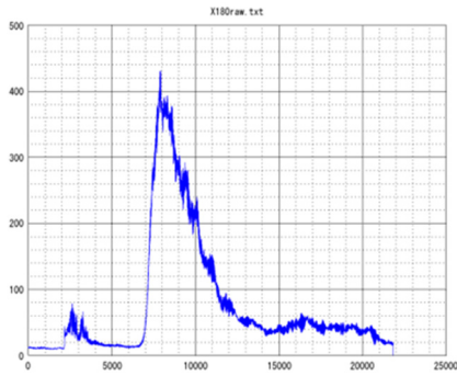
Figure 6: Growth and damping at the condition: N_B=2.3E+14 , 95% \xi correction.
