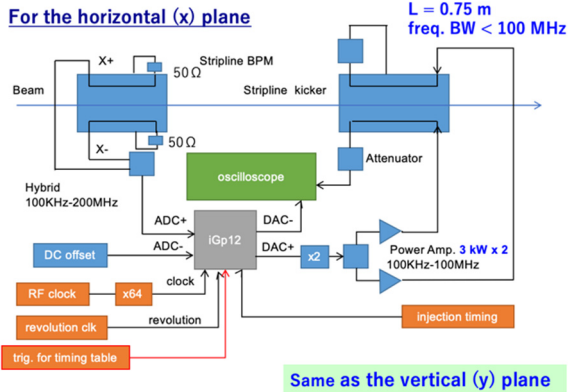
Figure 3: Schematic of the intra-bunch feedback system in the J-PARC MR.
