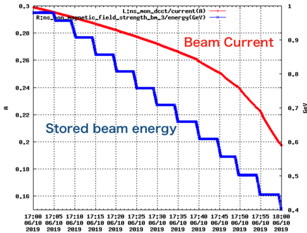
Figure 5: Electron beam deceleration by auto-generated ramping data. Stored beam energy (blue) and stored beam current (red).
