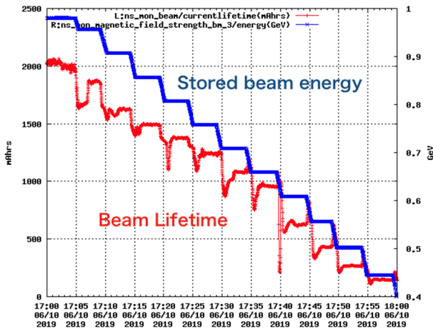
Figure 6: Electron beam deceleration by an auto-generated ramping data. Stored beam energy (blue) and beam lifetime I \cdot \tau (red).
