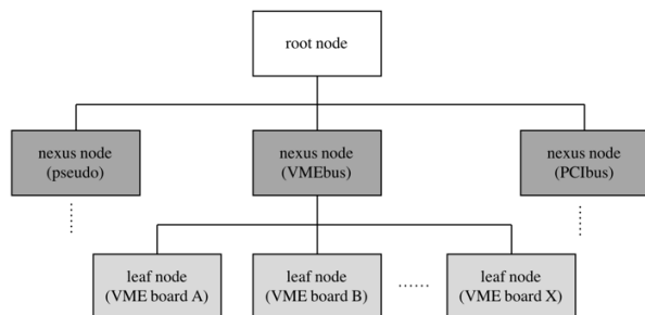
Figure 1: An example of the Solaris device tree.
