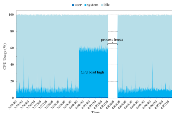
Figure 2: So-called “24 days problem” that the CPU load became high and running processes were frozen.
