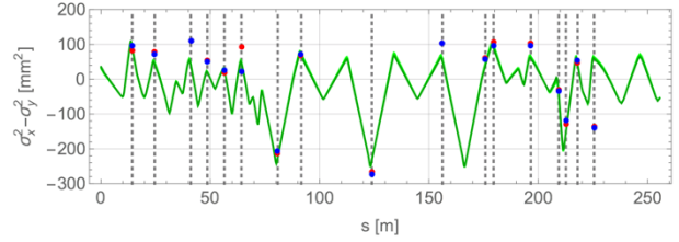
Figure 10: Fitted and calculated \sigma_x^2 - \sigma_y^2 . Red dots: front bunch, blue dots: rear bunch, green line: calculation with sad.
