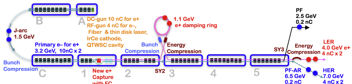
Figure 1: Schematic layout of the SuperKEKB injector linac.
