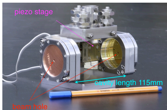
Figure 4: Cavity assembly.
