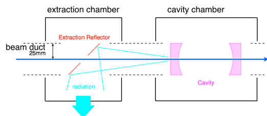
Figure 5: Chamber layout.
