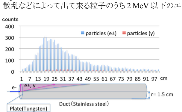
Figure 9: Histogram of the particle when the energy of the incident beam is 45 MeV.
