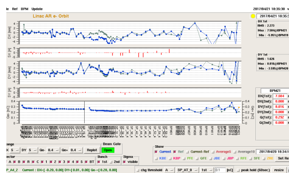
Figure 2: Typical beam orbit for PF-AR injection by using A1 thermionic electron gun. Top and middle lines indicate the horizontal and vertical beam orbits in mm units. Bottom line is the bunched beam charge in nC units.
