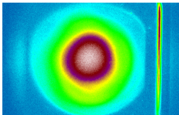
Figure 3: Spatial profile of the 12-nm soft XFEL beam. The horizontal full screen size is 17 mm.
