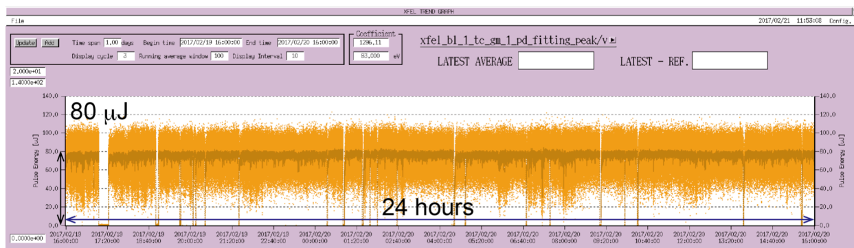
Figure 4: Trend graph of laser pulse energy at a 13-nm wavelength in 24 hours. The orange and brown dots indicate single shots and 100-shot-averaged, respectively. Stable laser pulses are delivered to experimental users for a long time.
