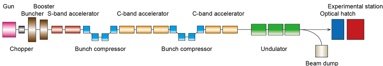
Figure 1: Schematic of the soft XFEL beamline of SACLA.
