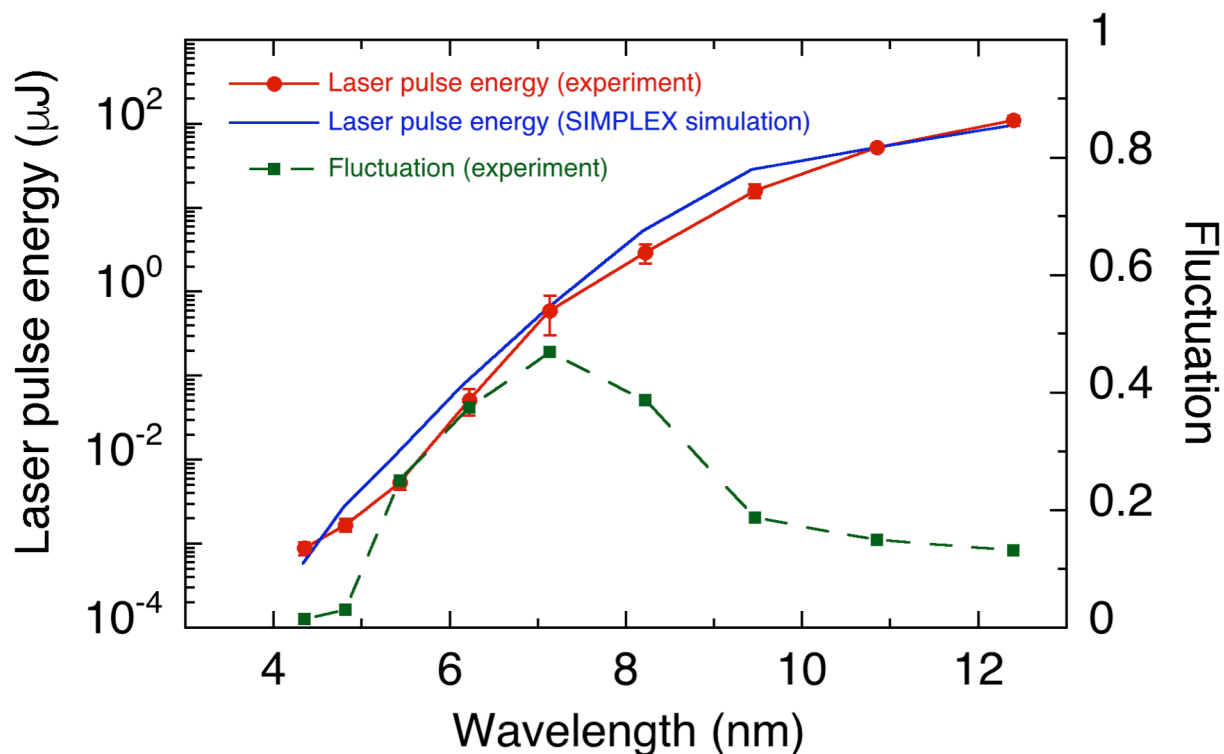
Figure 5: FEL gain curve of the SACLA-BL1. The radiation wavelength was scanned by means of changing the undulator's K-value.
